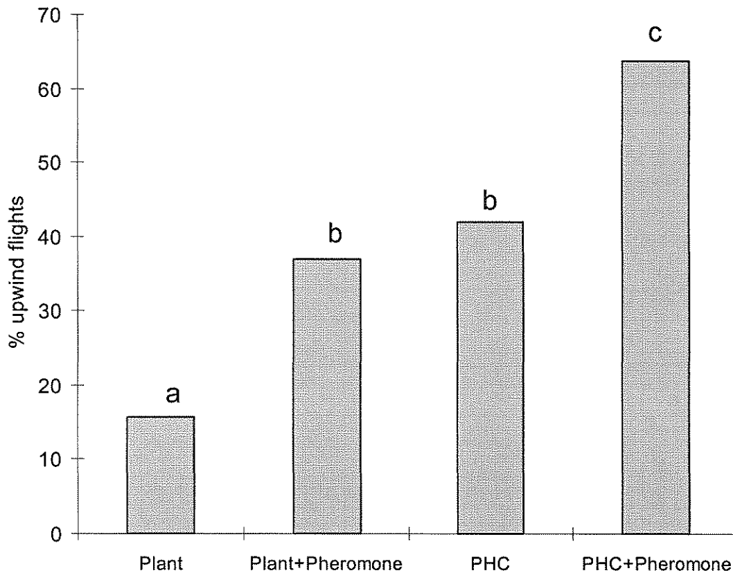
Fig. 3.5. Percentage of female parasitoids ( Aphidius ervi ) making direct flights in a wind tunnel towards uninfested broad bean plants, with or without an aphid sex pheromone lure, and towards bean plants infested with pea aphids ( A. pisum ), with and without an aphid sex pheromone lure attached. PHC = Plant/host complex.
