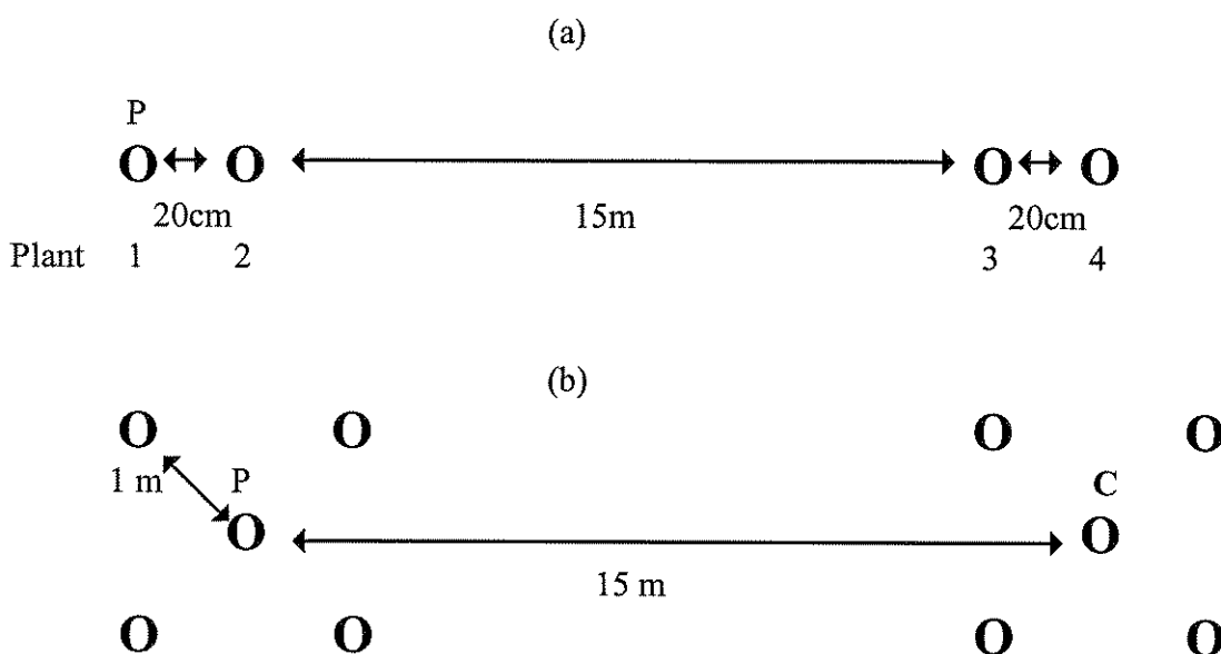
Fig. 4.1. Spatial arrangement of aphid trap plants used in the field spacing trials done in 1996 and 1997. P = plant with pheromone lure attached. C = control group.
