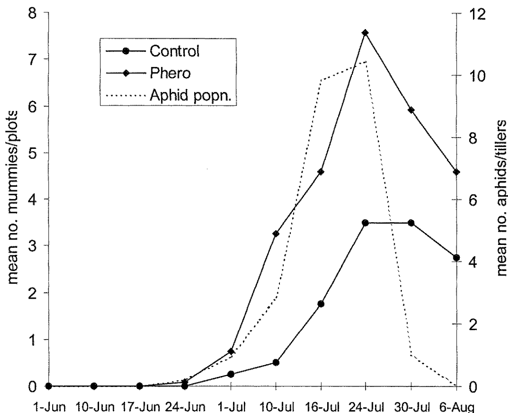
Fig. 4.3. Mean number of parasitized aphids (mummies) recorded at sampling points in winter wheat plots with and without aphid sex pheromone lures in 1996, together with the overall mean aphid density.
